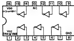
TC5020BP (TOSHIBA) C-MOS LOW-TO-HIGH VOLTAGE TRANSLATION INVERTER — TOP VIEW —
